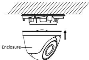
Figure 2-3 Secure the Camera/Enclosure/Trim Ring
