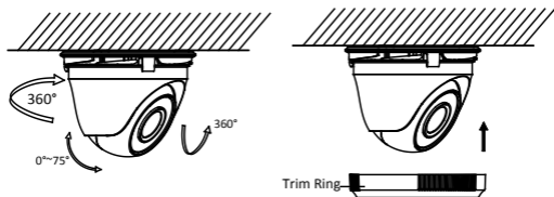
Figure 2-4 3-axis Adjustment
