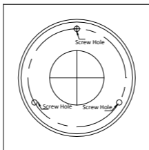
Figure 2-1 Drill Template of Type II Camera
