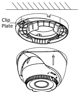
Figure 2-4 Install the Camera and the Enclosure
