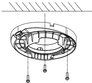
Figure 2-3 Fix the Mounting Base
