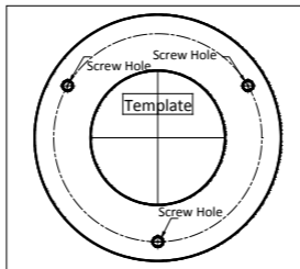
Figure 2-1 Drill Template of Type V Camera
