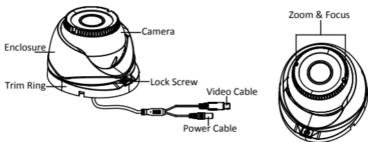
Figure 1-1 Overview of Camera
