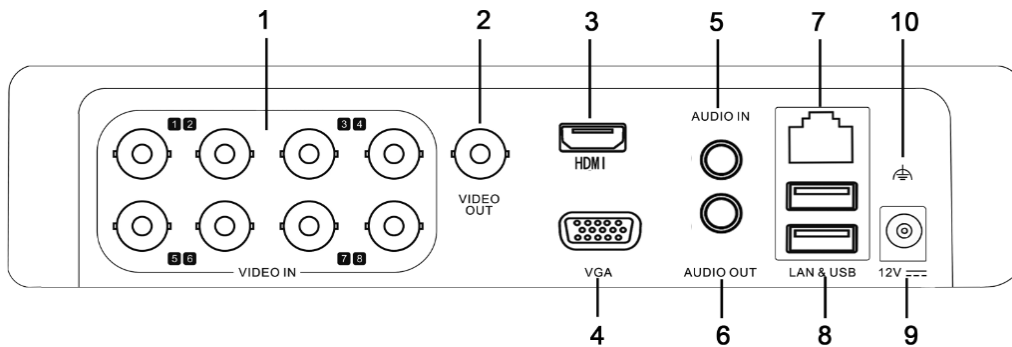
Figure 1.3 Rear Panel
