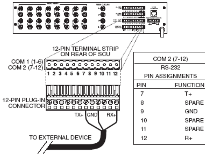
RS-232 port wiring. © Pelco
