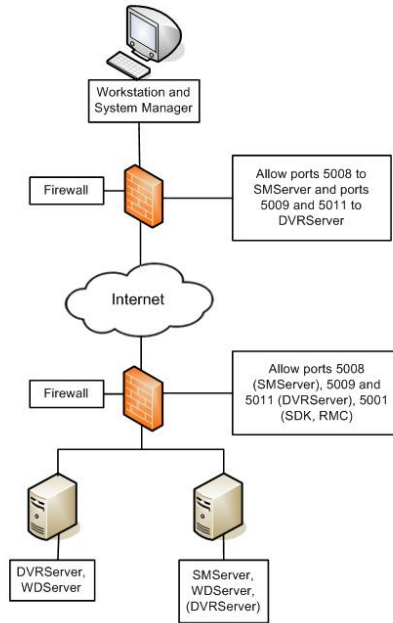
Figure 2 – DVMS System with firewalls
