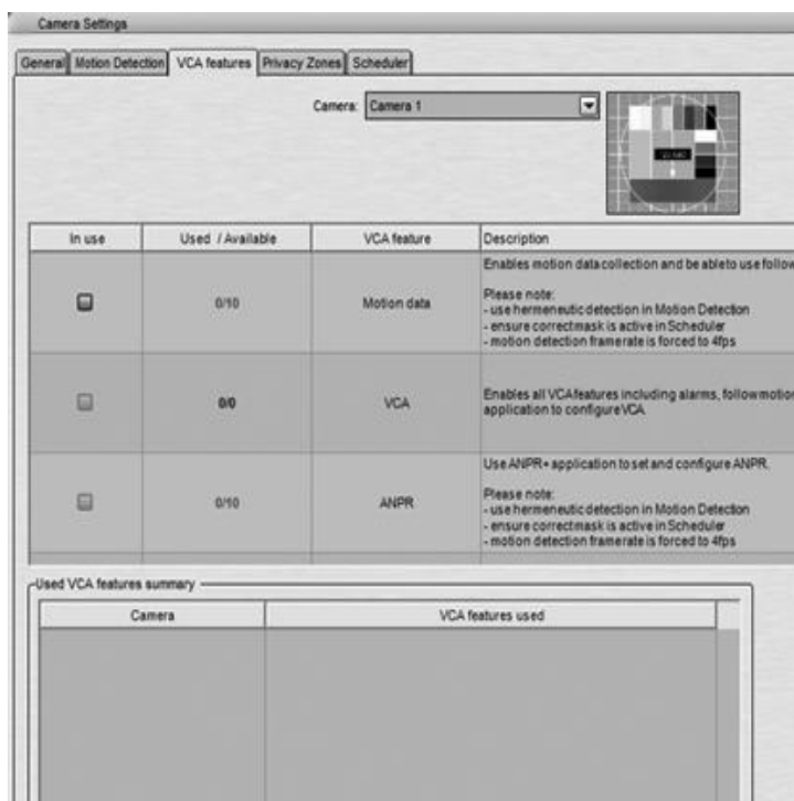
The VCA Features tab
